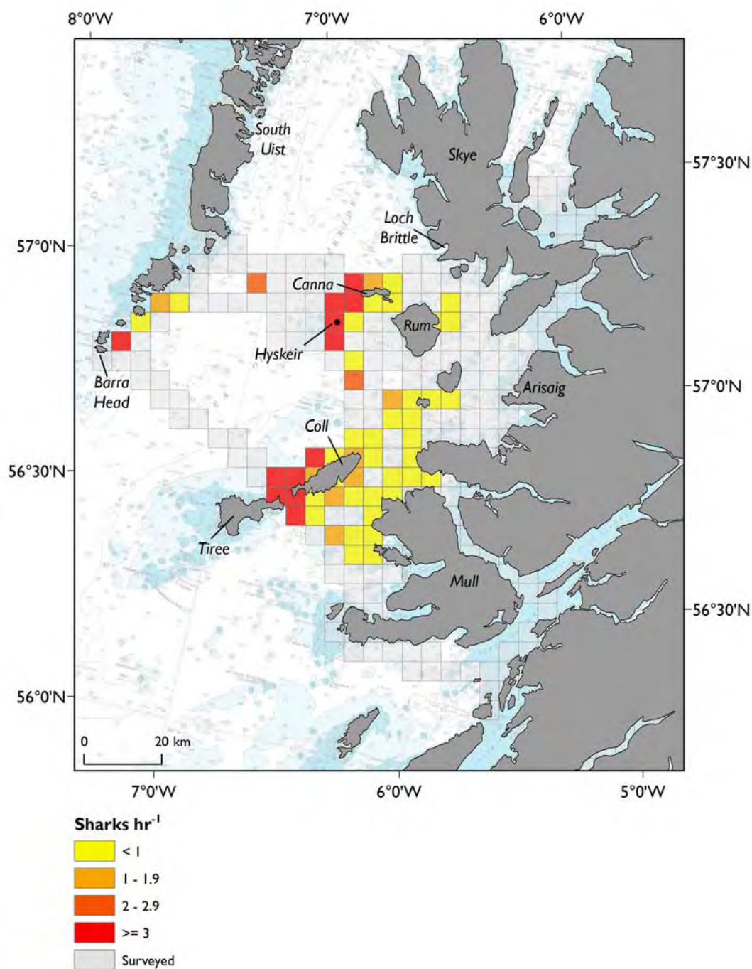
Figure 6: SPUE \text{h}^{-1} in the Sea of the Hebrides, 2002-2006, using a 25\text{km}^2 grid ( 5\text{km} \times 5\text{km} )
